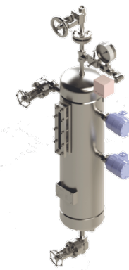
API Plan 52/53A
